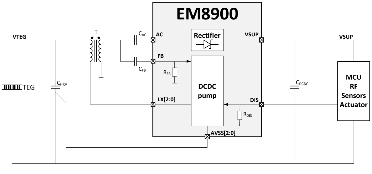
Figure 2-1: Block Diagram
