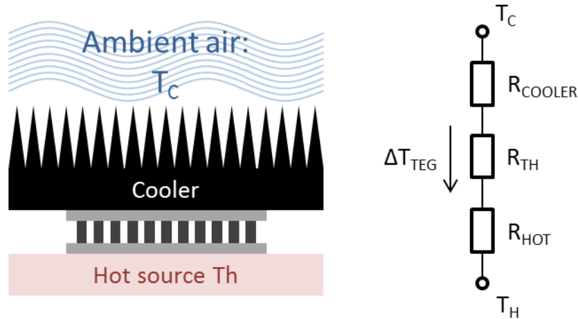
Figure 3-1: Thermal Structure
