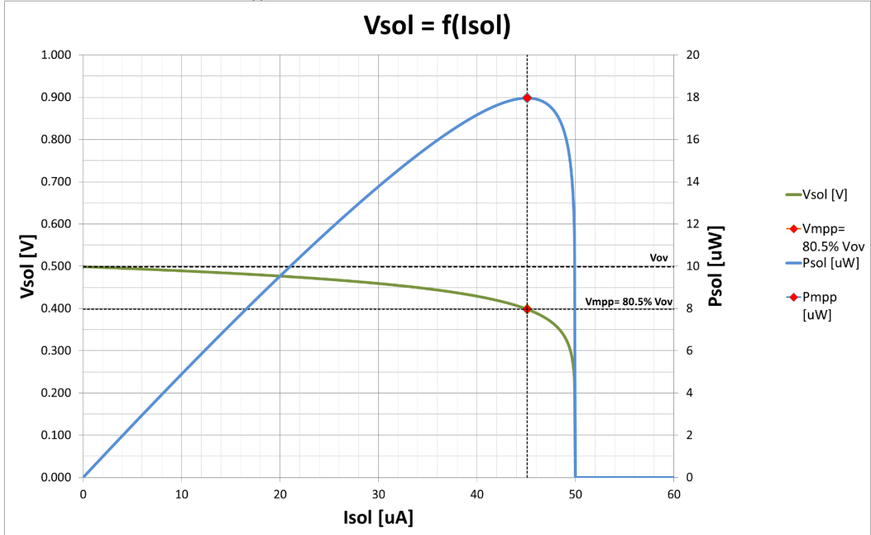
Figure 2: V=f(I) Curve of a Solar Cell
