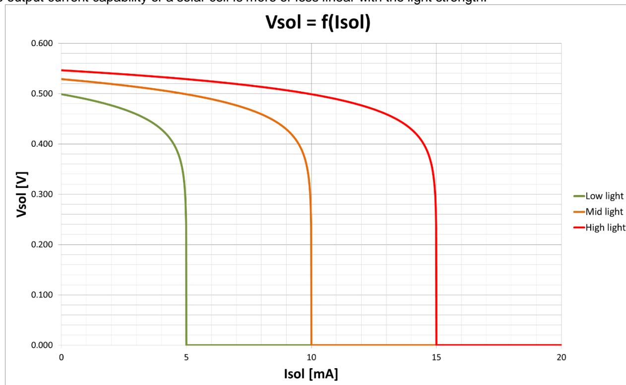
Figure 4: V=f(I) Solar Cell Curves for Different Light Strengths
