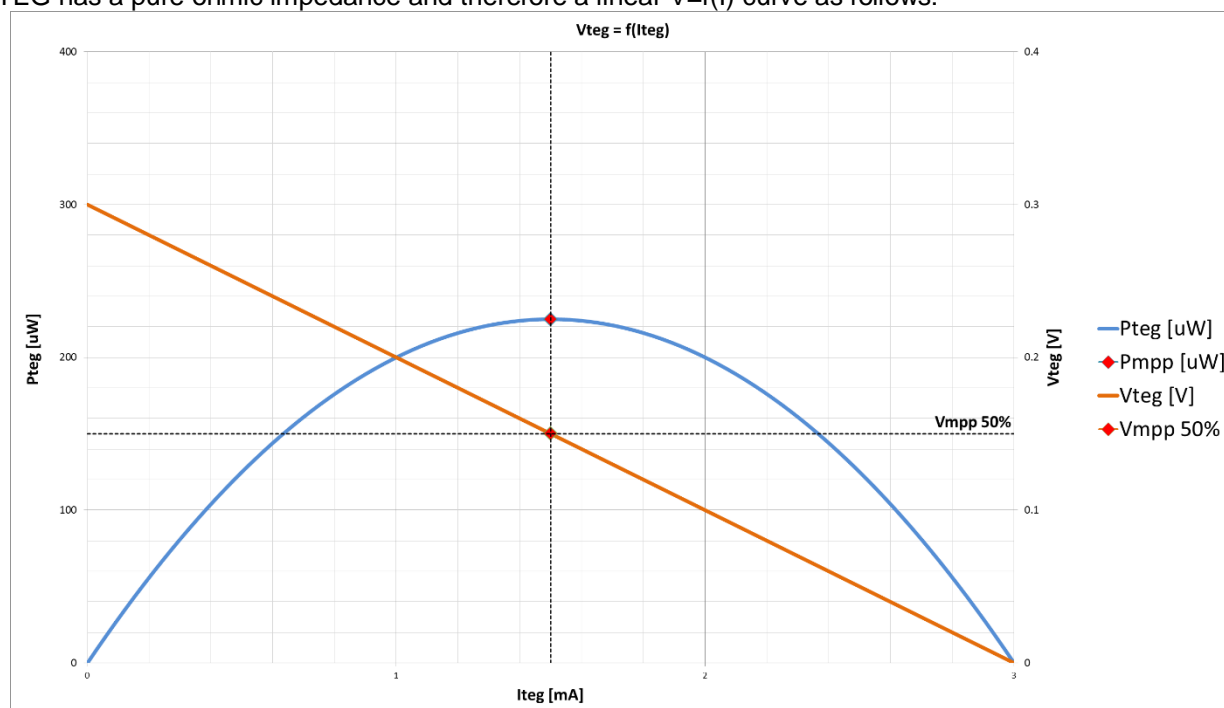
Figure 1: V=f(I) Curve of a TEG
