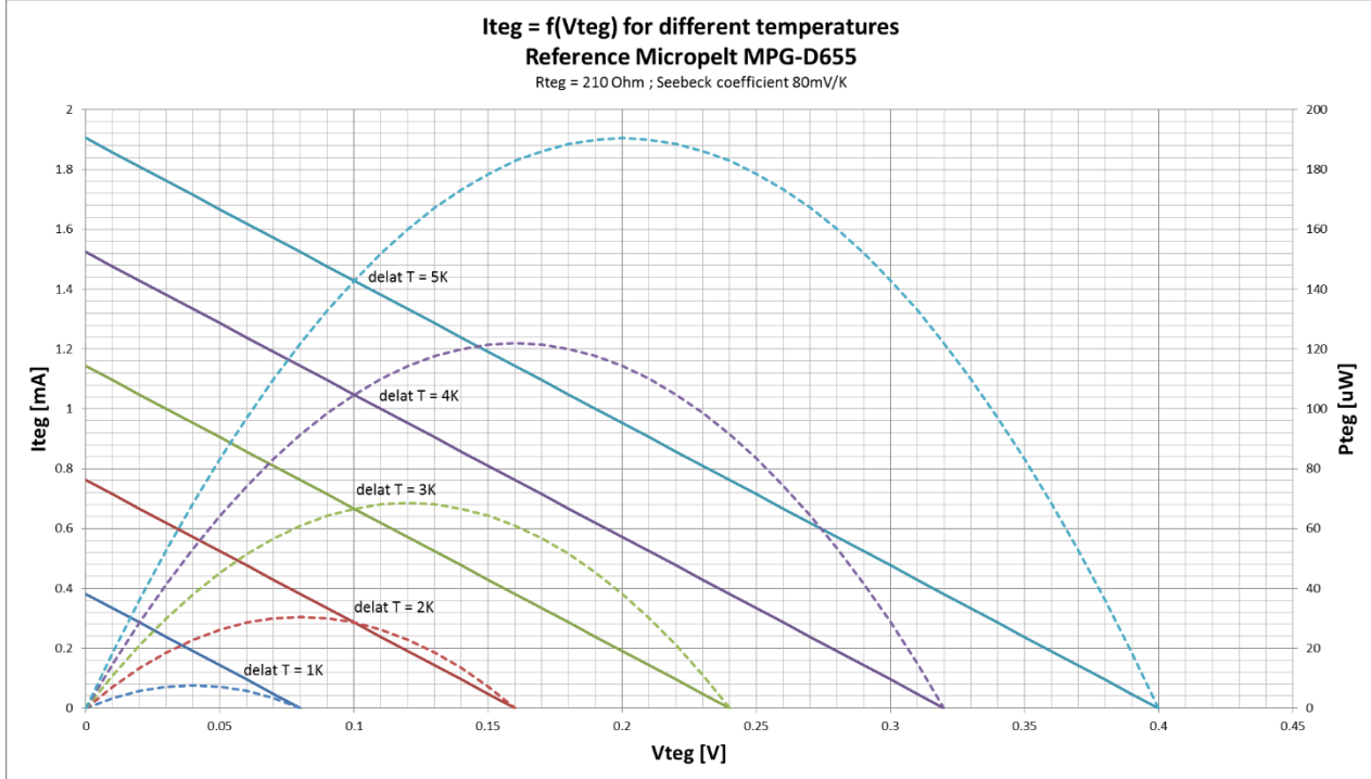
Figure 3: V=f(I) Curve of a MPG-D655 for Different Delta Temperatures
