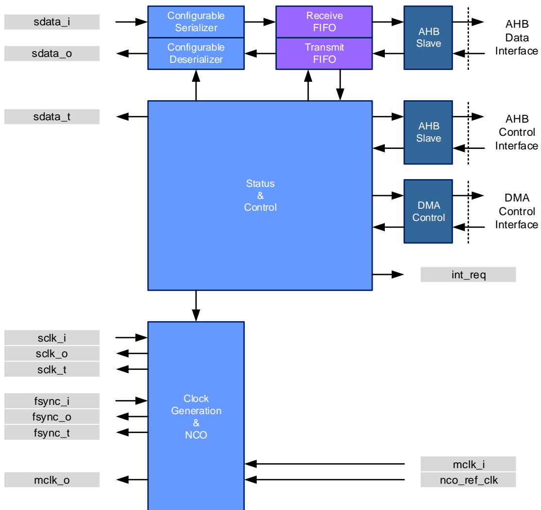
Figure 8-6: Architecture of the serial audio interface I2S/TDM
