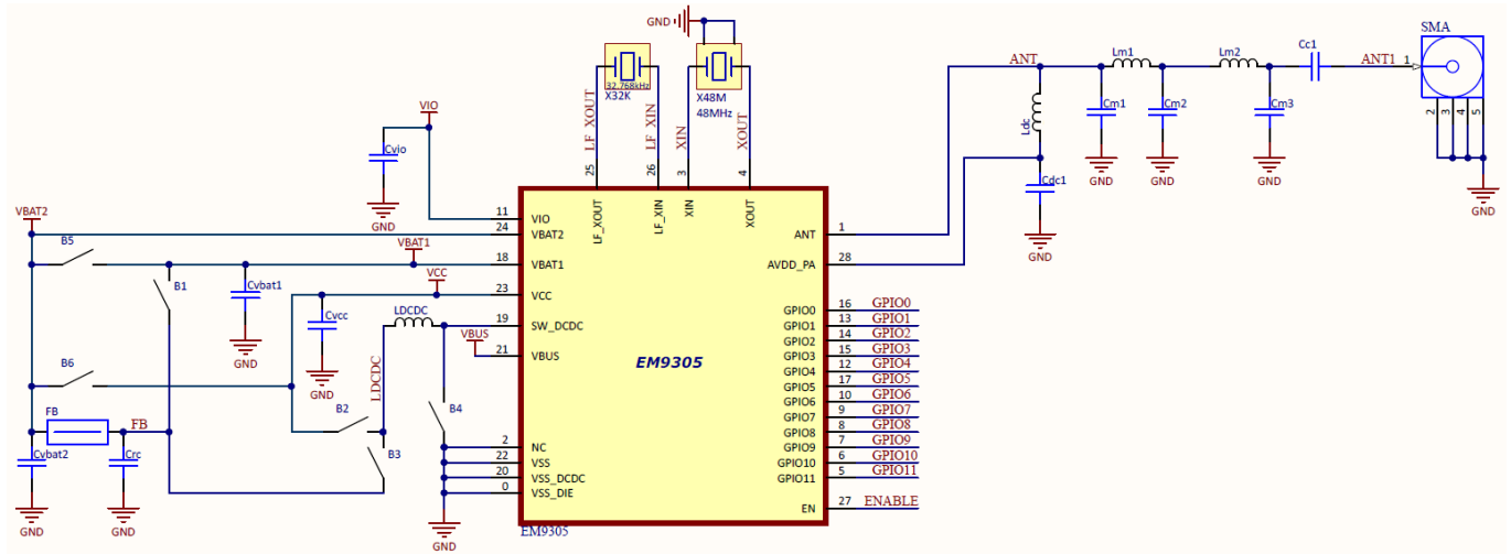
Figure 12-1: QFN General Reference Design Schematic
