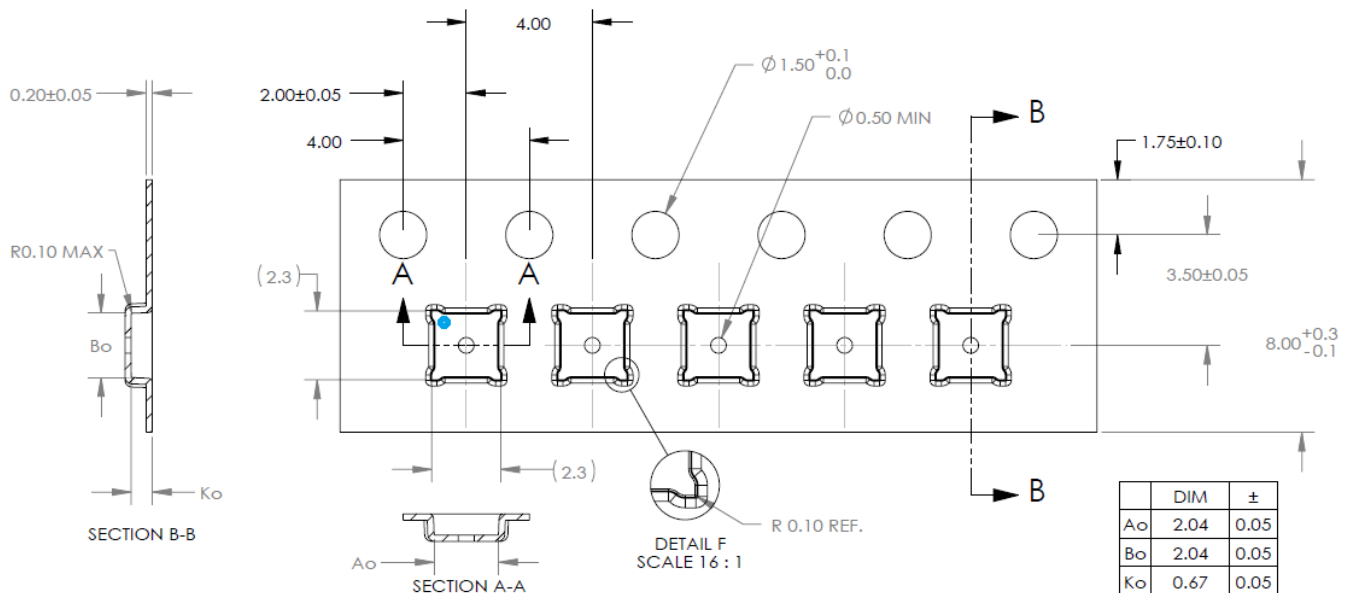
Figure 14-4 Tape & Reel diagram. Blue dot shows pin A1 orientation on WLCSP tape (All dimensions are in millimetres)
