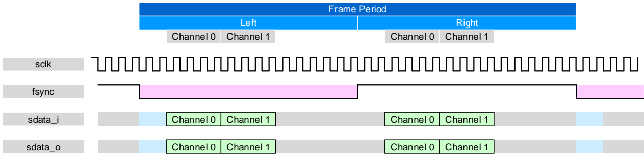
Figure 8-11: TDM in I2S frame format
