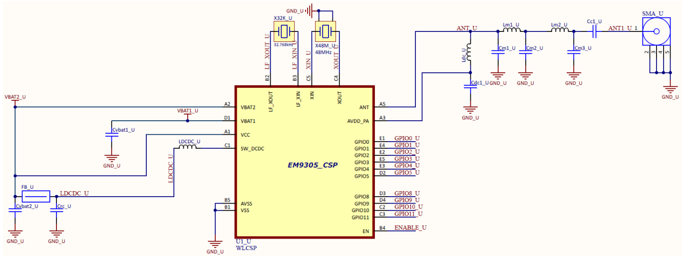
Figure 12-5: WLCSP Step-up Reference Design Schematic
