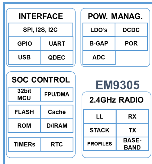
Figure 1-2: Hardware Architecture
