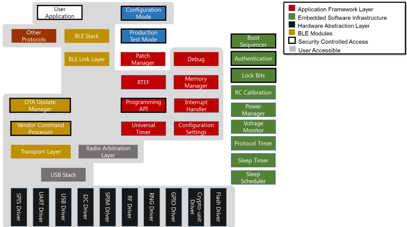
Figure 10-1: Software architecture
