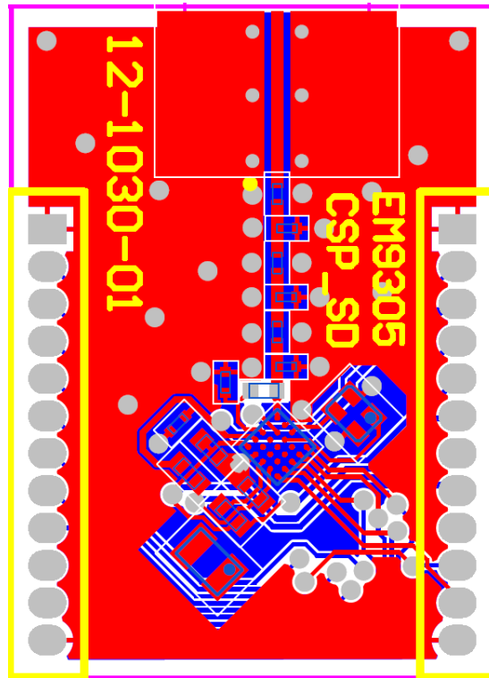
Figure 12-4: WLCSP Step-down Reference Design Layout
