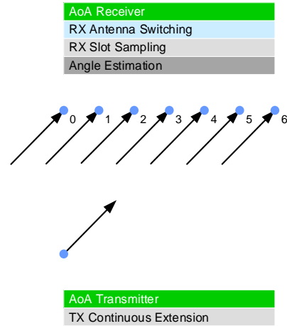
Figure 7-8: Angle-Of-Arrival (AOA) system representation
