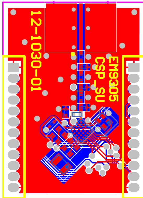
Figure 12-6: WLCSP Step-up Reference Design Layout
