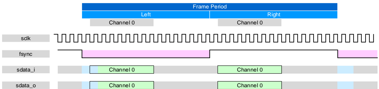
Figure 8-8: I2S frame format
