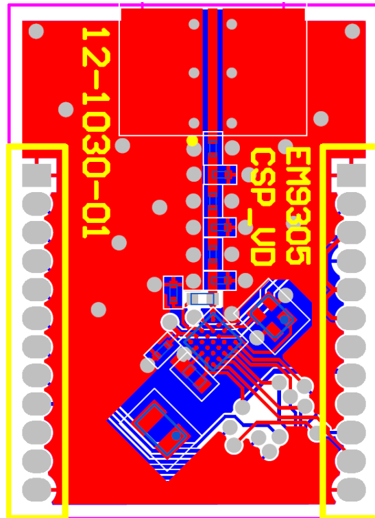
Figure 12-8: WLCSP Voltage Multiplier Reference Design Layout
