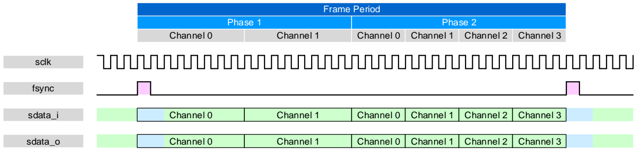
Figure 8-7: TDM frame format
