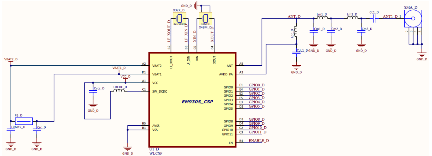
Figure 12-3: WLCSP Step-down Reference Design Schematic
