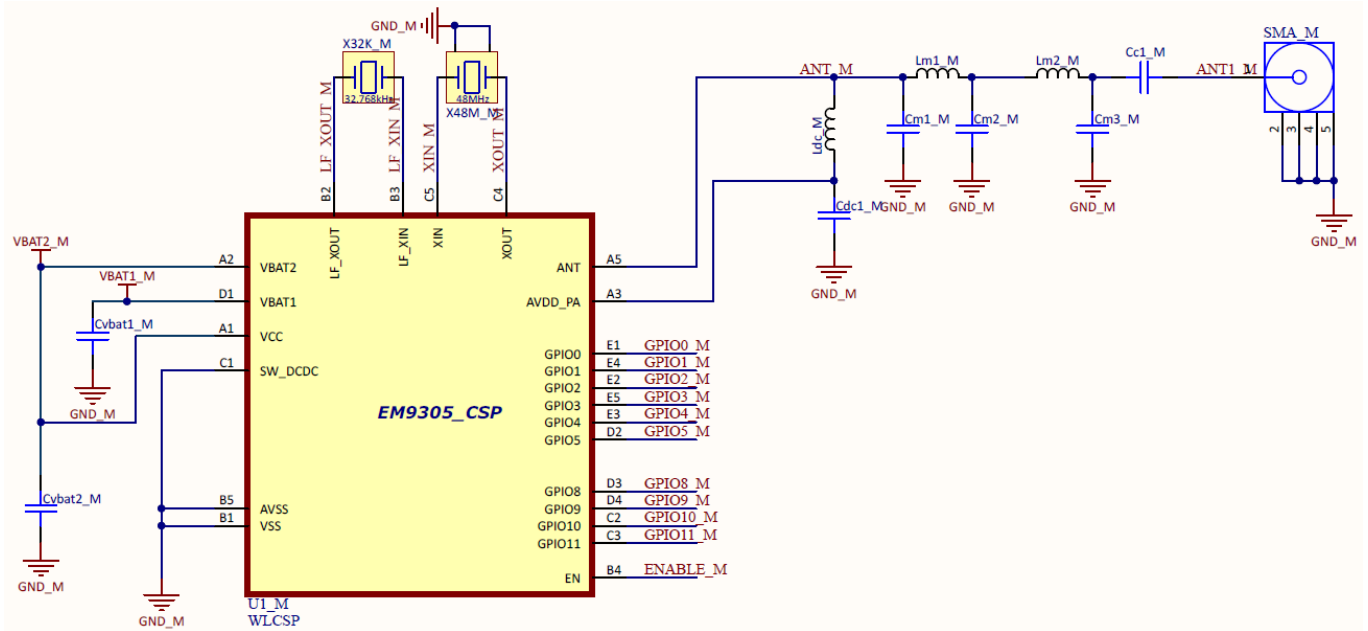
Figure 12-7: WLCSP Voltage Multiplier Reference Design Schematic
