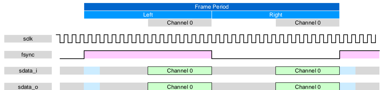
Figure 8-10: Right-Justified frame format
