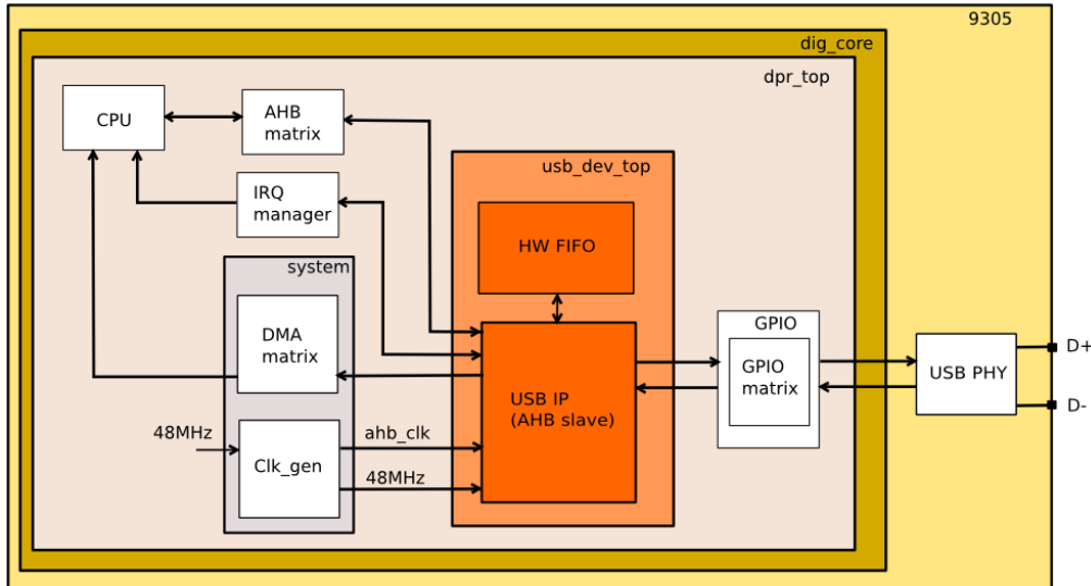
Figure 8-23: USB system level integration
