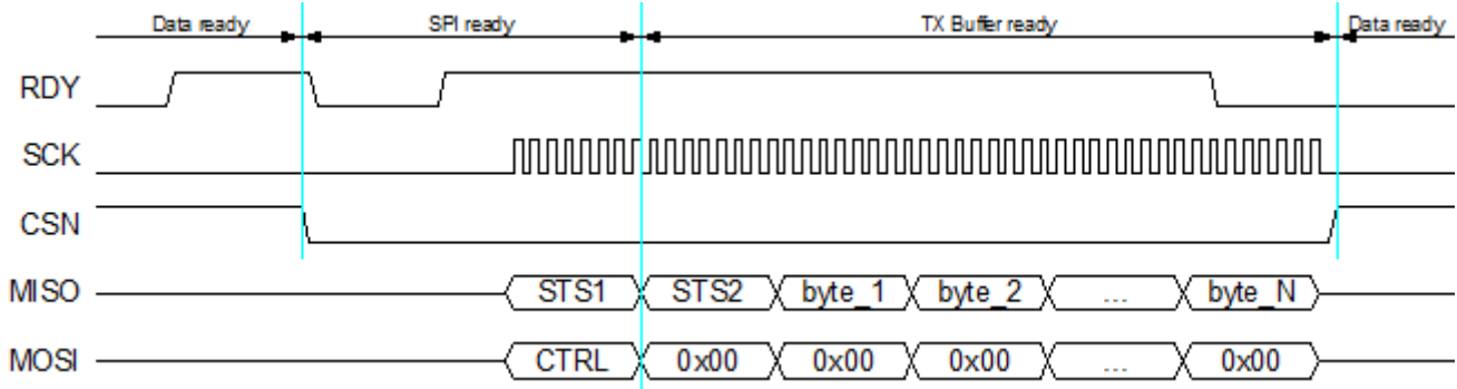
Figure 8-21: SPI control, data ready in RX buffer
