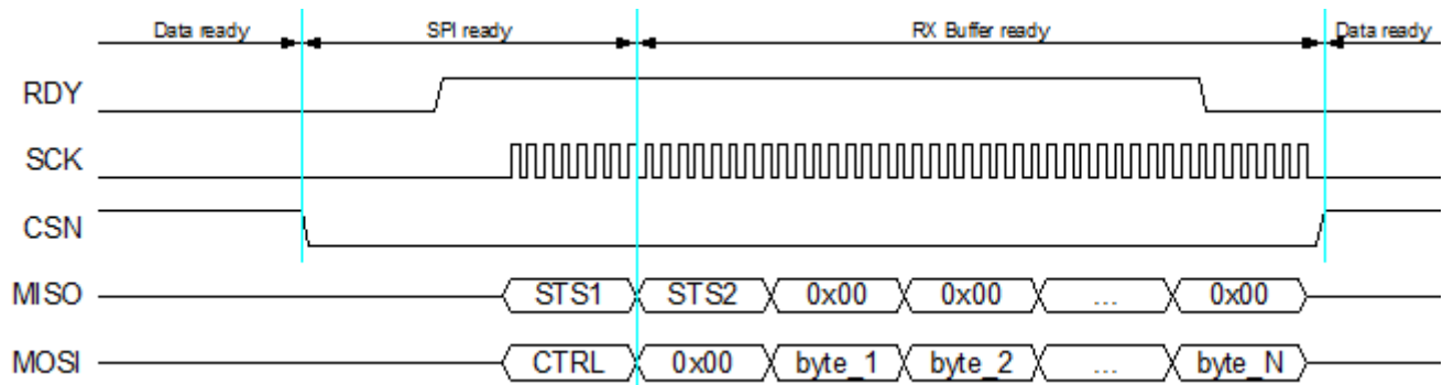
Figure 8-20: SPI control, slave ready for transactions
