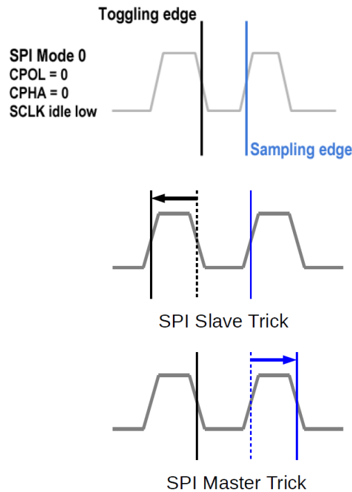
Figure 8-18: SPI trick to increase maximum speed
