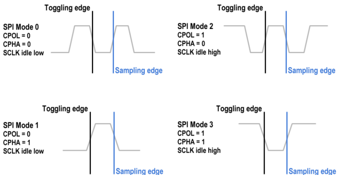
Figure 8-17: SPI modes
