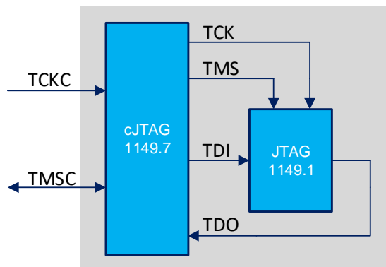
Figure 8-13: cJTAG (IEEE 1149.7) interface
