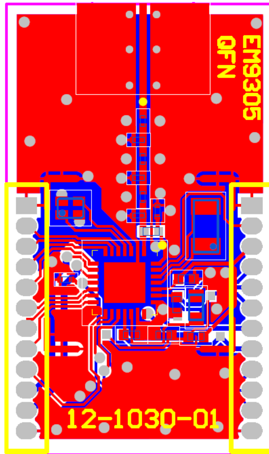
Figure 12-2: QFN General Reference Design Layout
