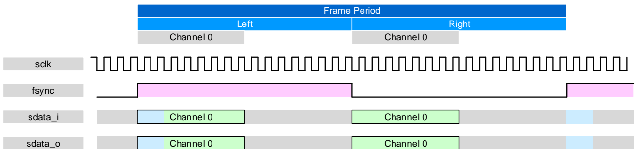
Figure 8-9: Left-Justified frame format
