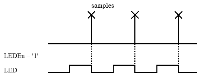
Figure 8-16: QDEC LED enable before sample
