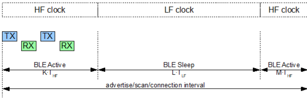
Figure 8-22: Protocol timer and sleep timer cooperation
