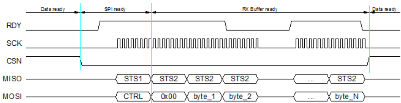
Figure 8-19: SPI Slave write transaction with active flow control using RDY
