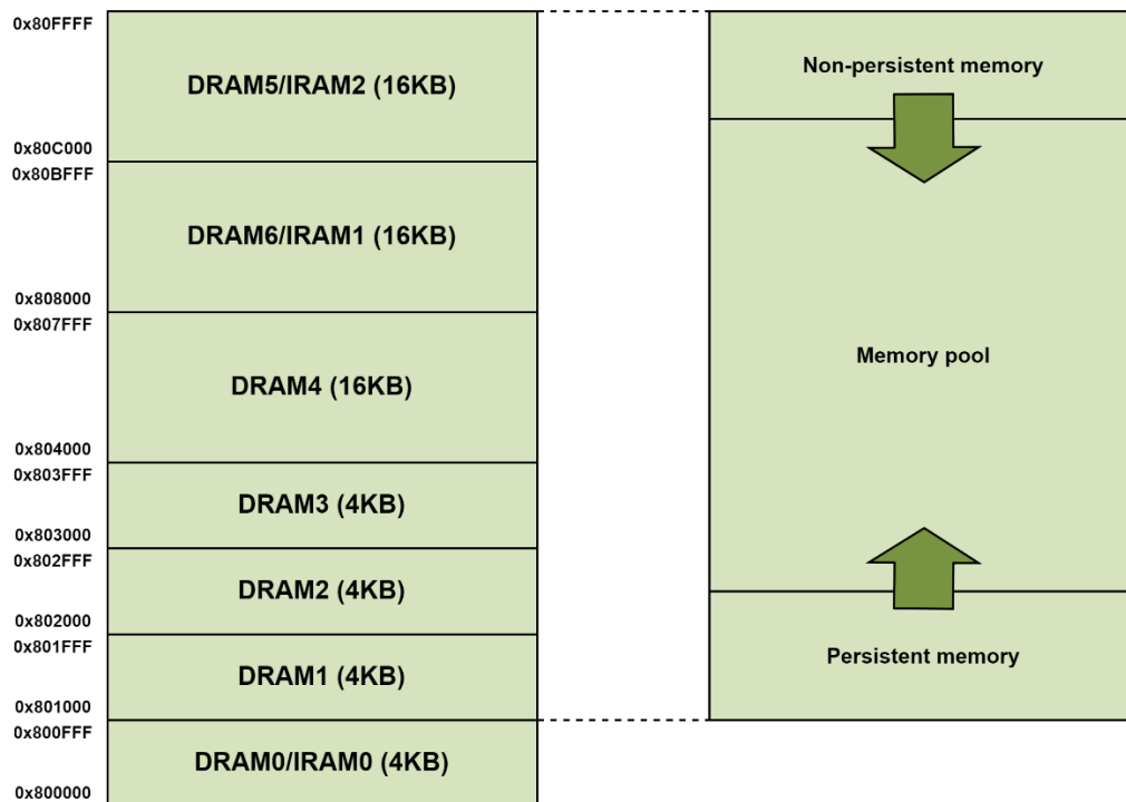
Figure 10-3: Data address space and persistence strategy
