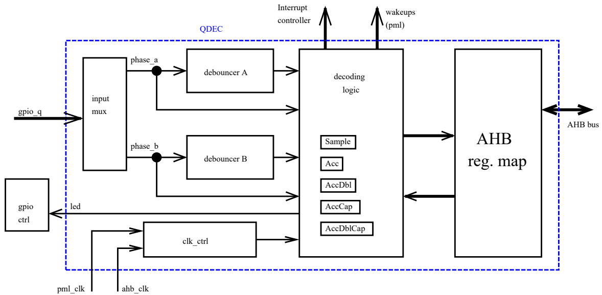
Figure 8-15: QDEC block diagram
