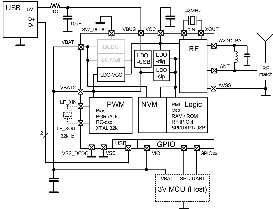
Figure 1-7: USB configuration
