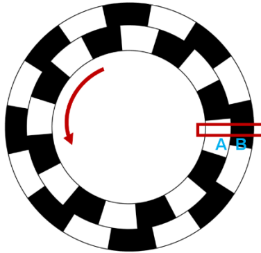
Figure 8-14: Rotary decoder with corresponding logic states for A and B signals
