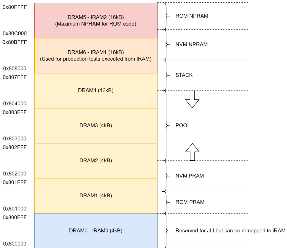
Figure 10-2: RAM address space
