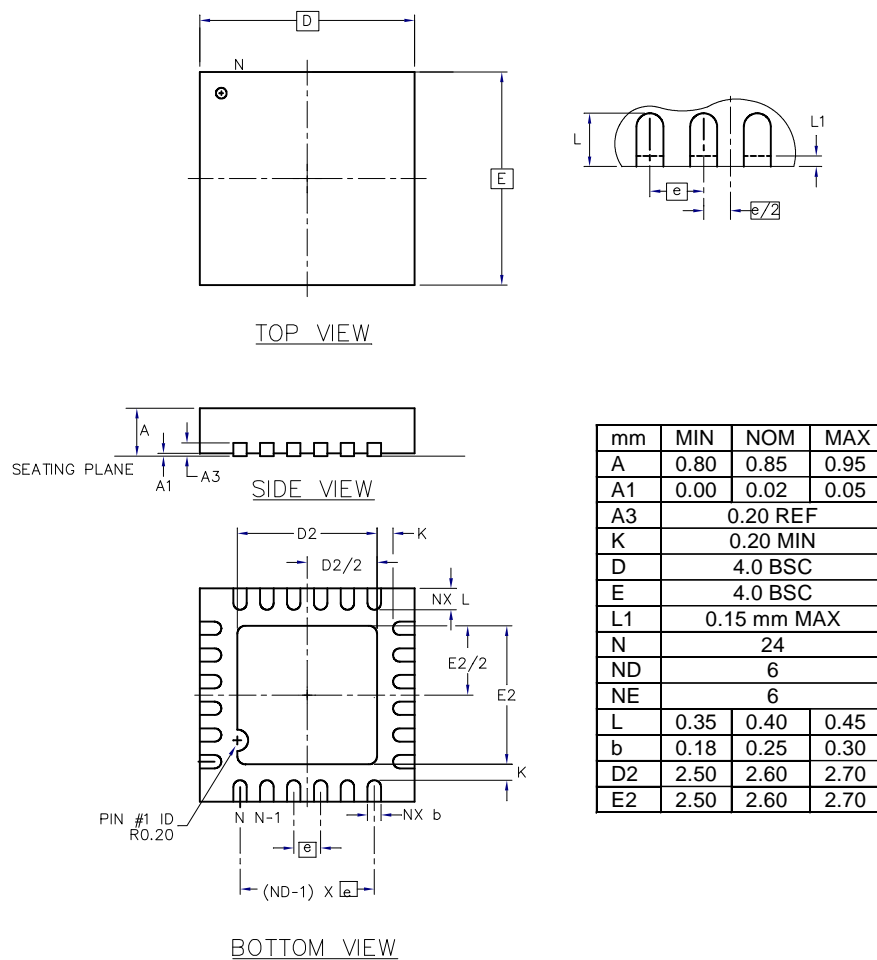
Figure 6.1: Package information
