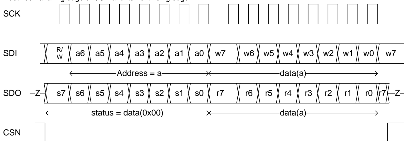
Figure 3.5 Raw SPI transaction
