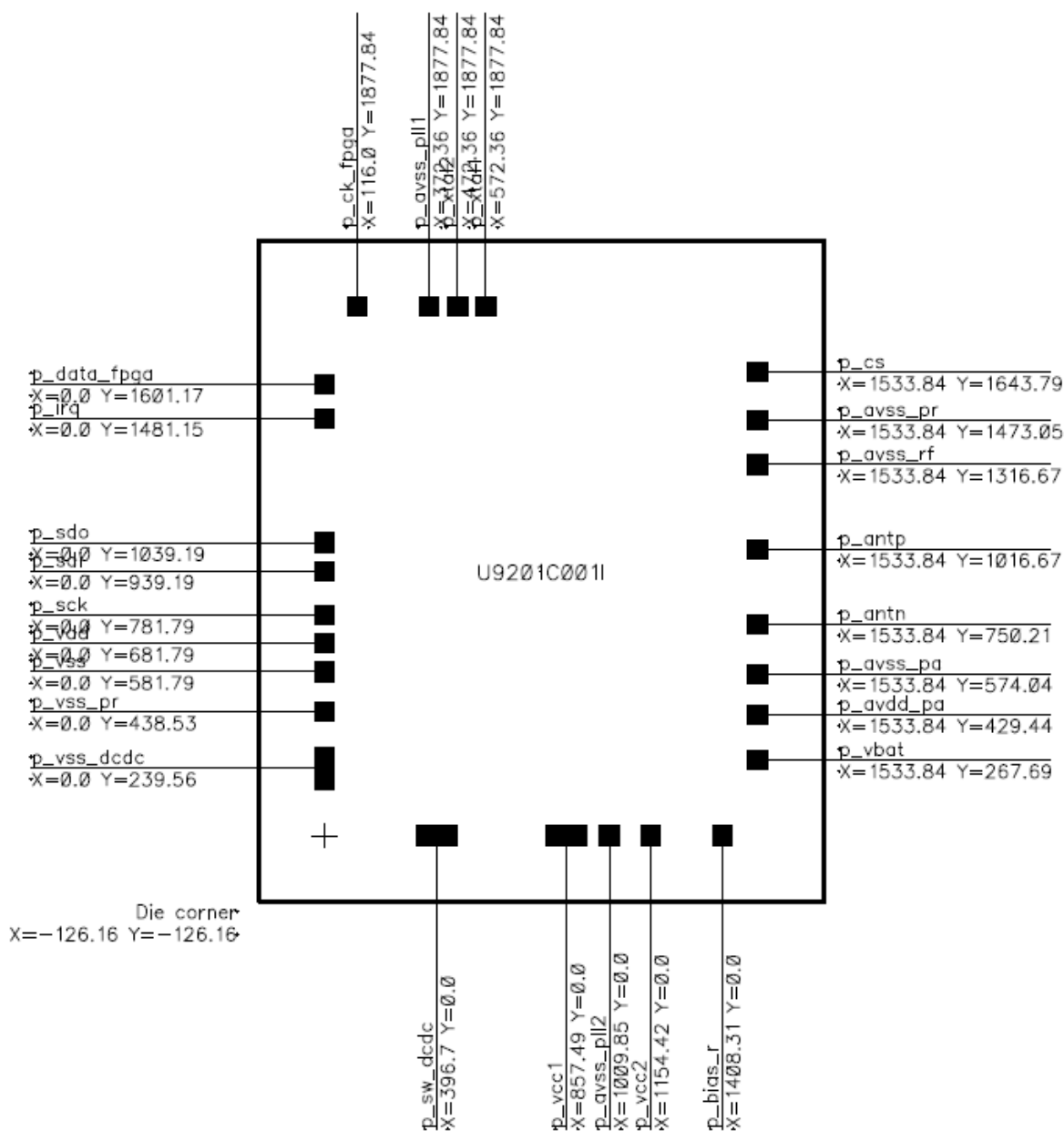
Figure 5.5: Pad location diagram
