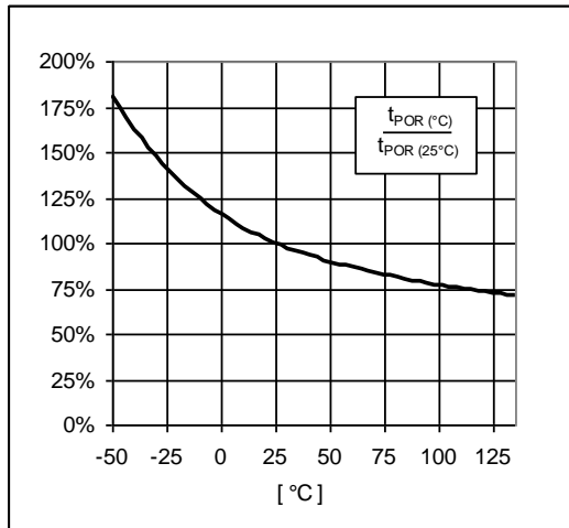
Reset Timeout Period t_{POR} vs. Temperature (normalized with respect to t_{POR} 25^\circ\text{C} )
