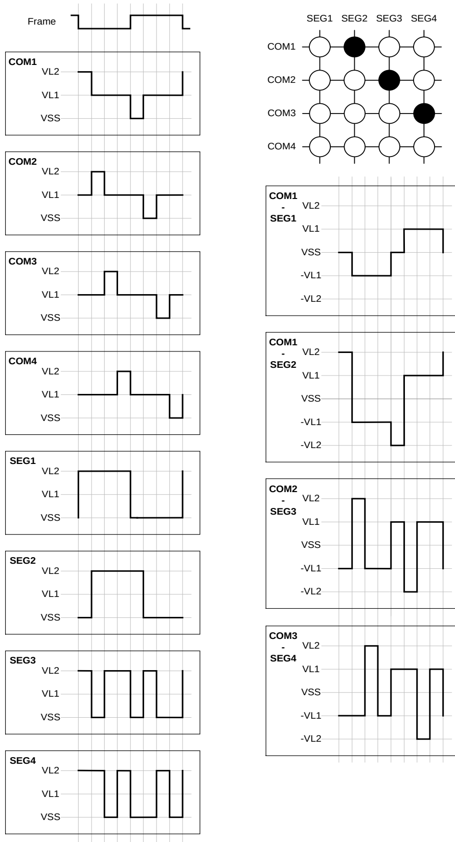
Figure 2-6 : LCD Driver Waveforms – Mux4 & Bias ½ mode
