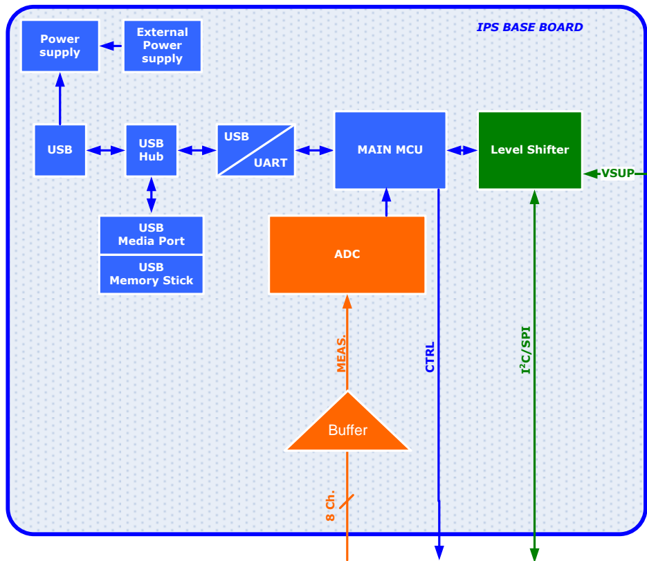
Figure 9-1: Base board simplified block diagram
