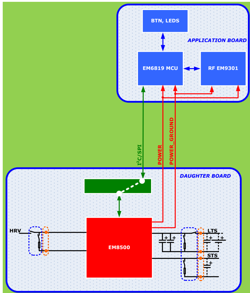
Figure 5-4 EMDVK85xx Stand-alone Mode with default application board
