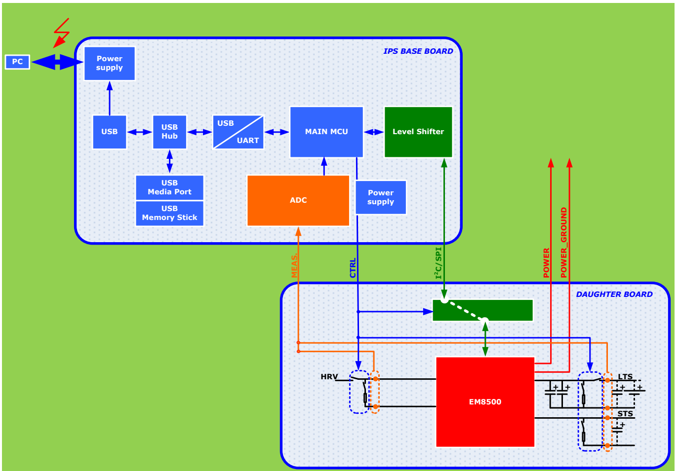
Figure 5-2 EMDVK85xx Configuration Mode
