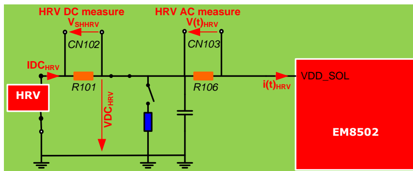
Figure 8-5: HRV measurements variant EM8502
