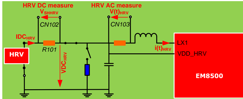
Figure 8-4: HRV measurements variant EM8500
