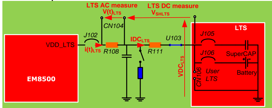
Figure 8-6: LTS measurements
