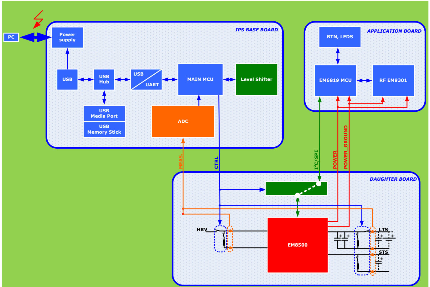
Figure 5-3 EMDVK85xx Application Mode
