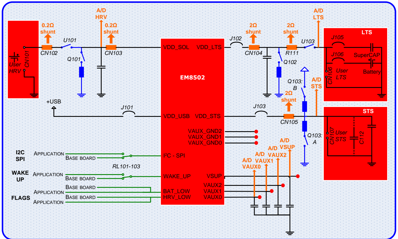
Figure 8-2: Daughter board simplified schematic variant EM8502
