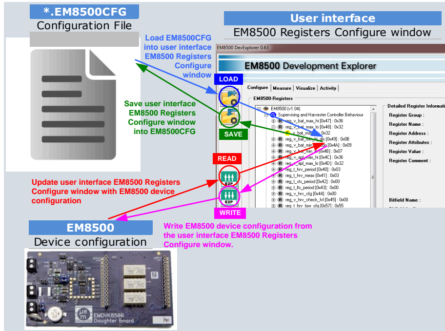
Figure 10-4 EM8500 DevExplorer configuration flow description
