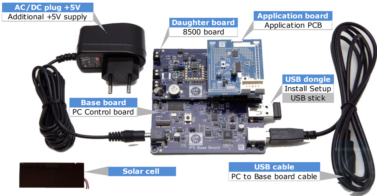
Figure 3-1 EMDVK8500 deliverables
