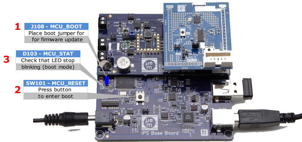
Figure 4-1 Configure boot mode (firmware update)
