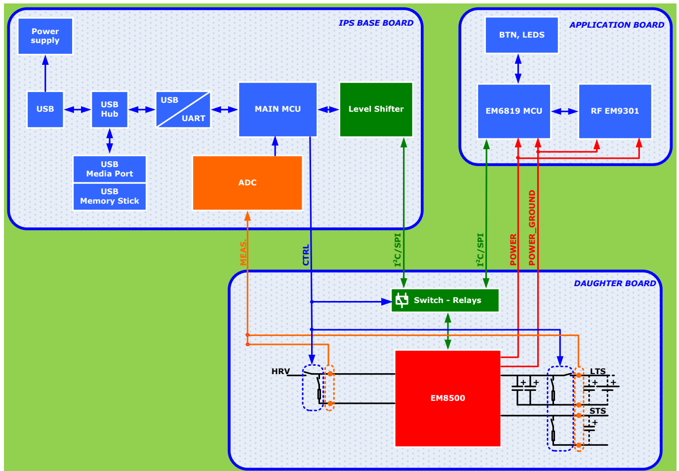
Figure 5-1 EMDVK85xx System Architecture
