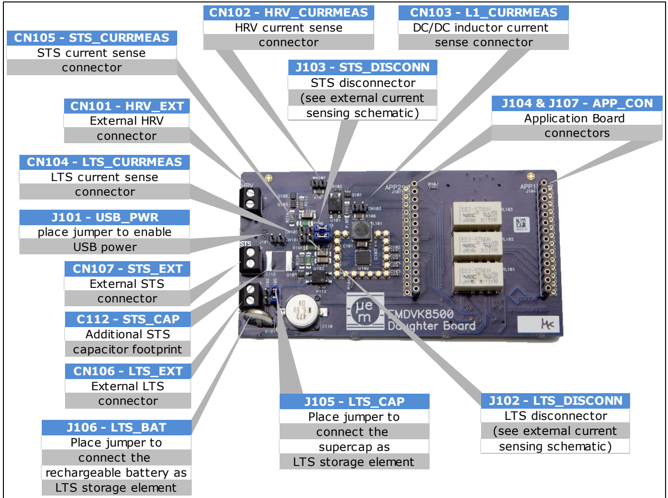
Figure 8-3: Daughter board description
