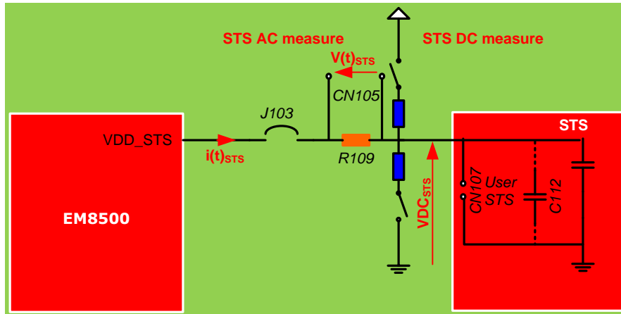
Figure 8-7: STS measurements
