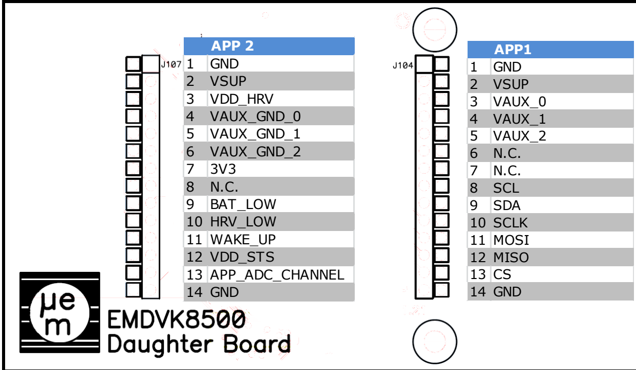
Figure 6-1 EMDVK85xx Daughter board – application connections APP2 (J107) and APP1 (J104) - top view
