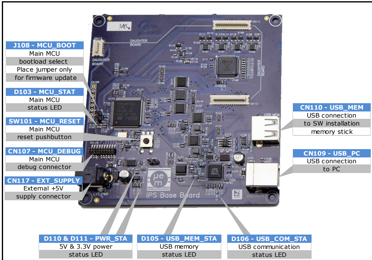
Figure 9-2: Base board description
