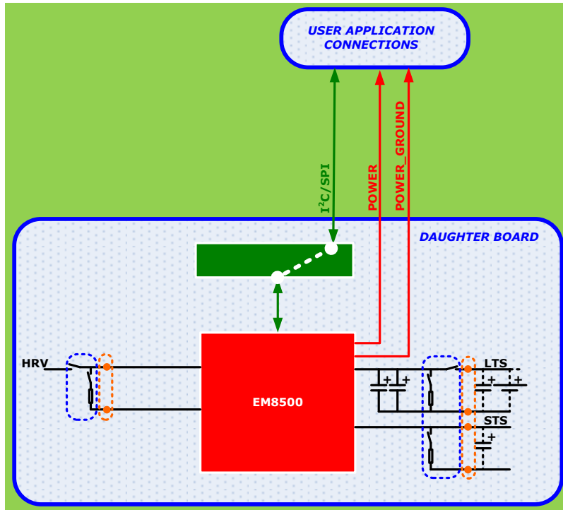
Figure 5-5 EMDVK85xx Stand-alone Mode with user application connections
