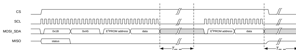
Figure 7-9 SPI multi-byte transaction for writing the E²PROM
