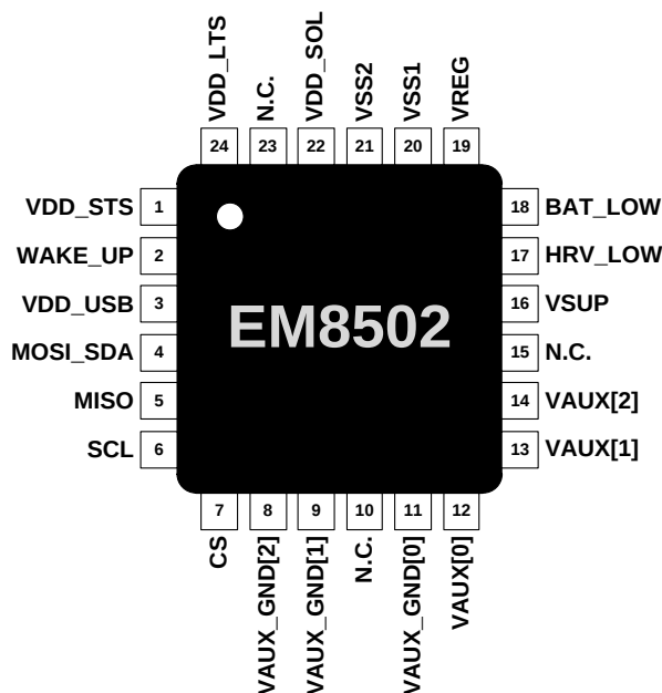
Figure 1 EM8502 QFN24 pins location
