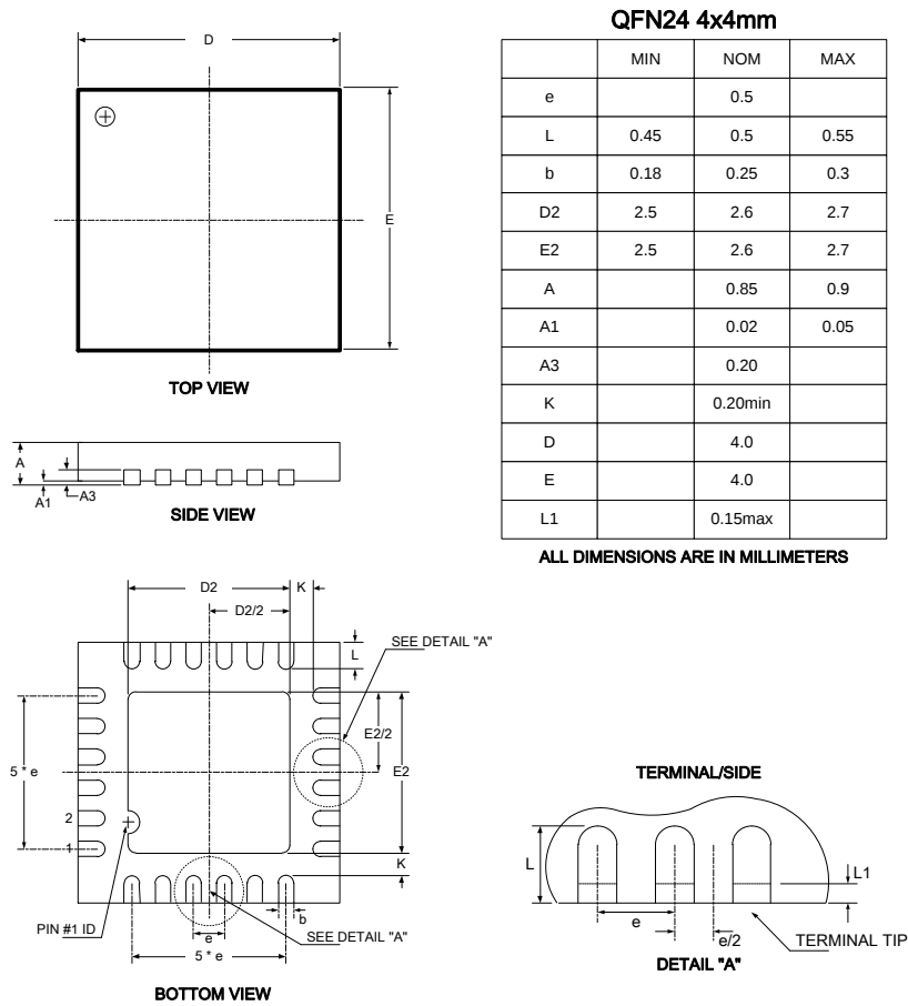
Figure 10-1 QFN24 Mechanical Information
