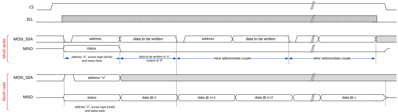
Figure 7-5 Multi register access transaction
