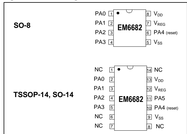
Figure 2. Pin Configuration
