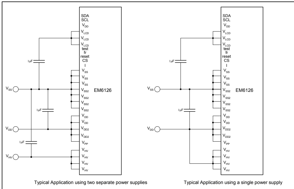
Figure 39: Power Supply connection
