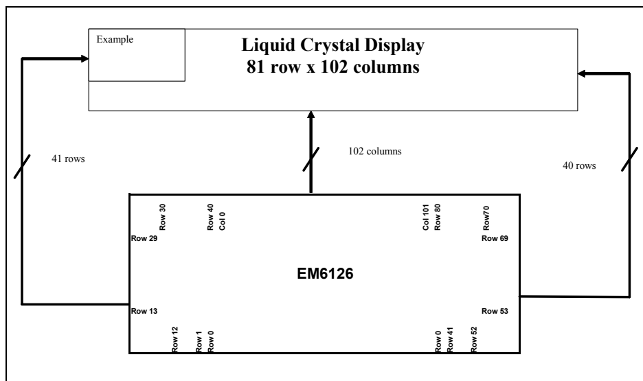
Figure 40: Connection between EM6126 and LCD for the application example
