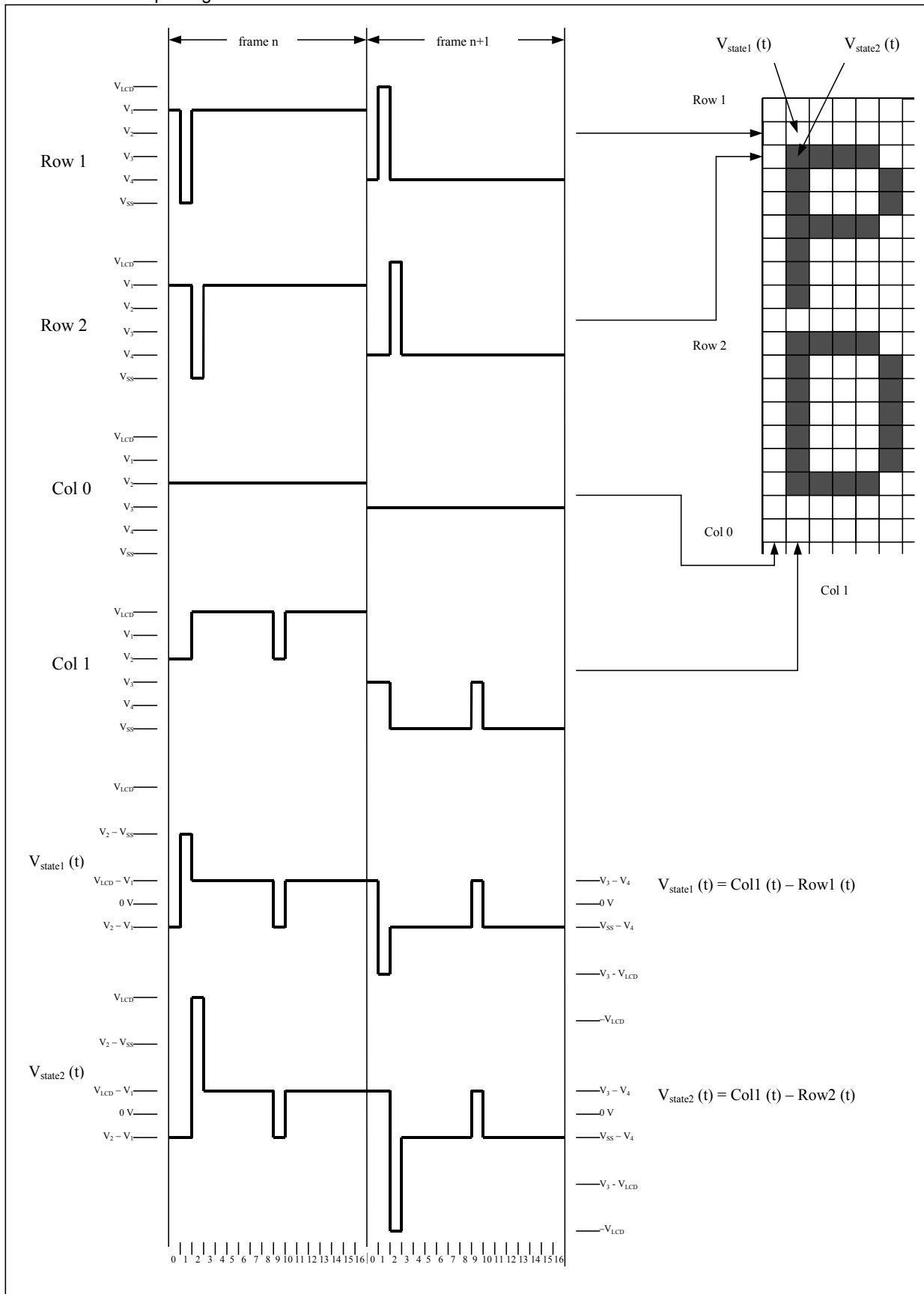
Row and Column Multiplexing Waveform EM6126 Mux = 17
