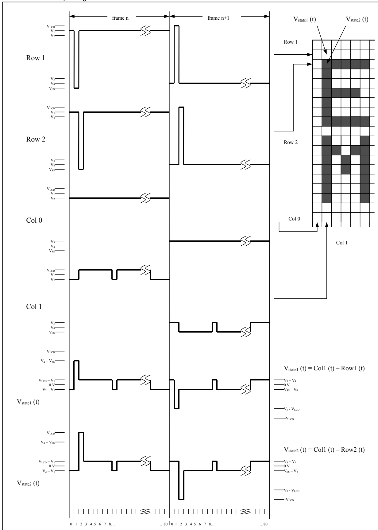
Row and Column Multiplexing Waveform EM6126 Mux = 81
