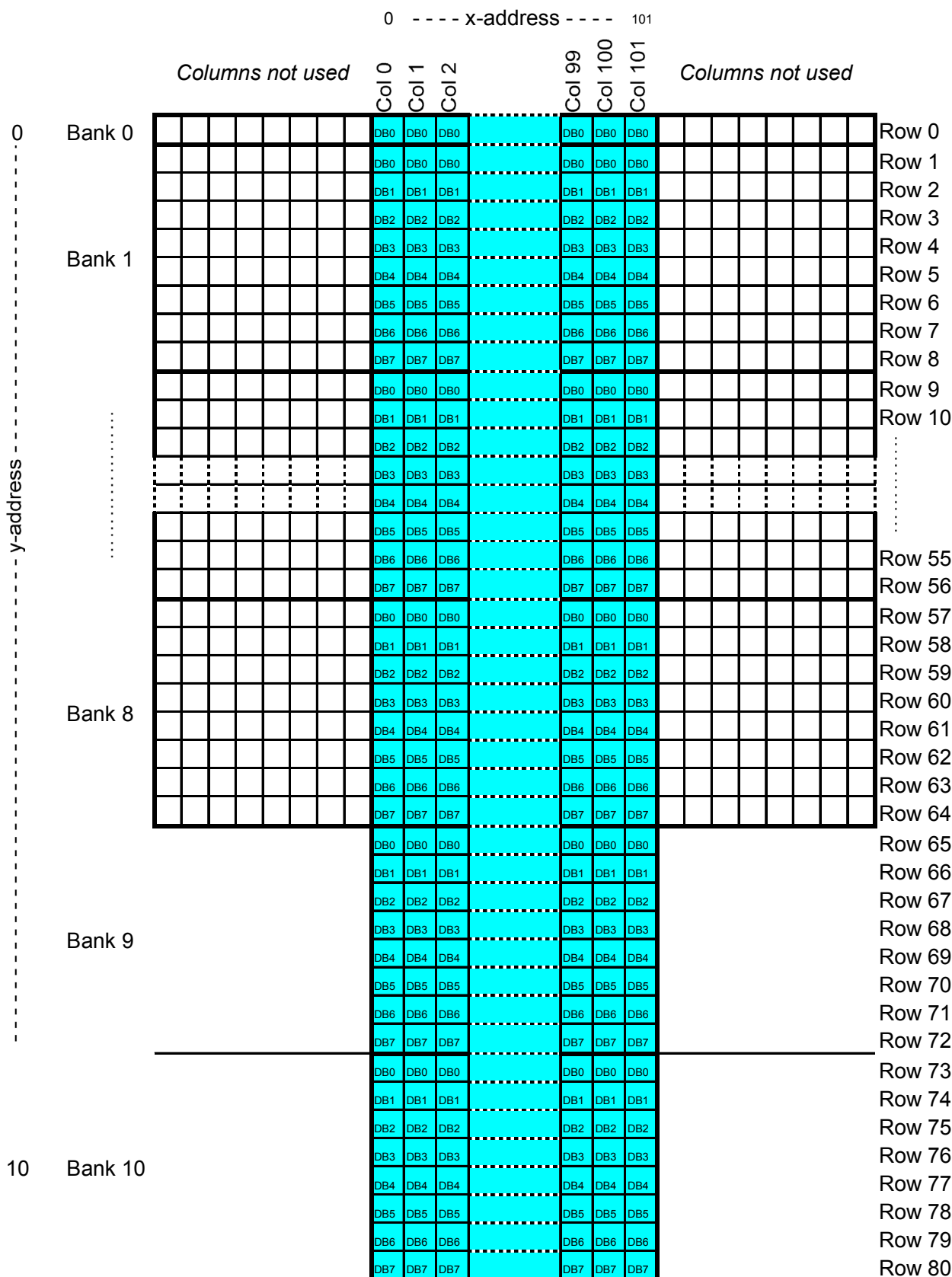
Figure 15: DDRAM description with Mux Mode = 1 and LSB = 1
