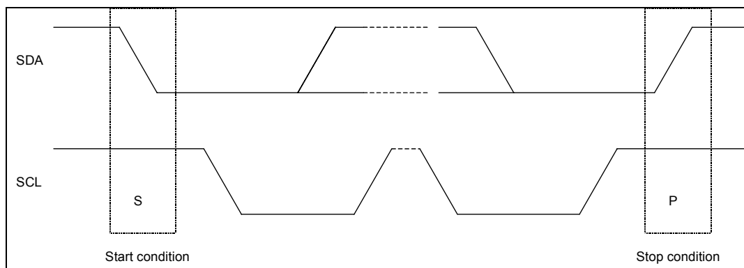
Figure 4: I 2 C start and stop conditions
