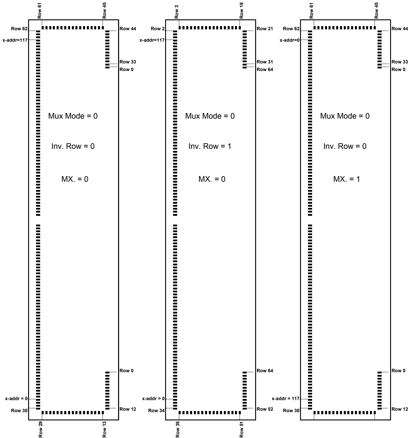
Figure 34: LCD output pads configuration in mux 65 depending on Inv. Row and MX
